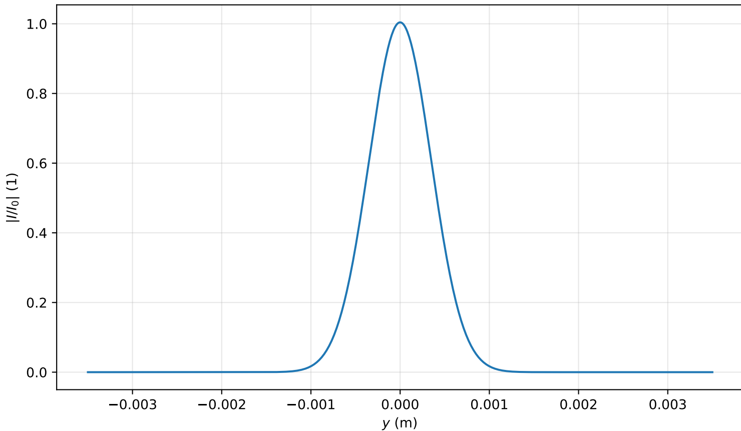
Intensity profile I(x=0, y, z=0.080)/I_0 , \text{Pin}=0.9\text{Pcr} , artificial time
